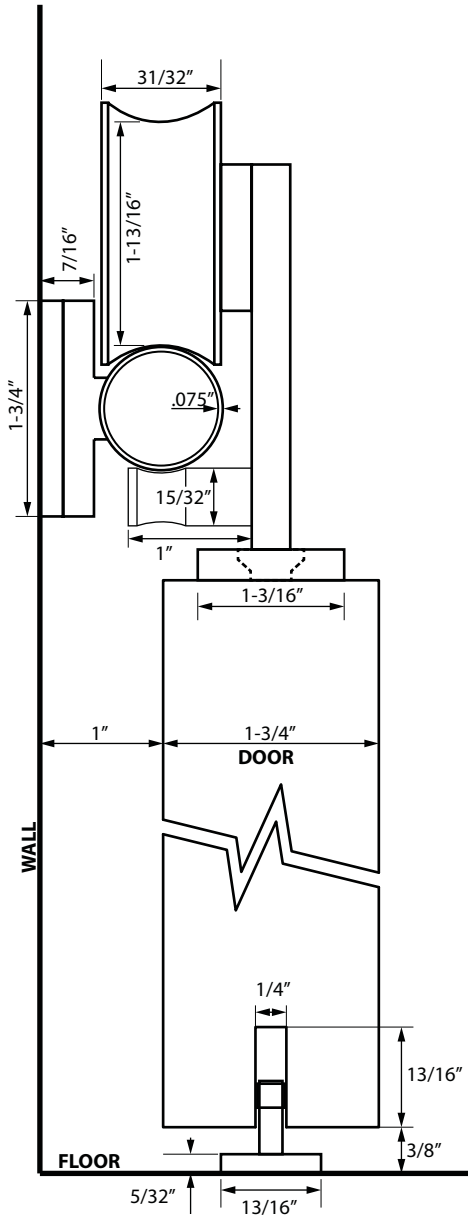
SIDE VIEW
